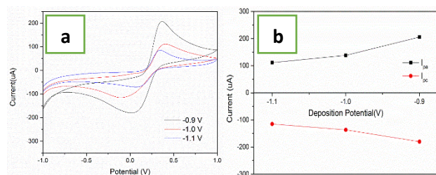
Fig. 5 (a) Cyclic voltammogram of (\text{FeCN}_6)^{3-} at ZnO modified electrode deposited at -0.9 V, -1.0 V and -1.1 V at deposition temperature of 60 °C. (b) Plot of anodic and cathodic peak currents behavior of ZnO modified ITO obtained at various deposition potential
