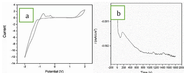
Fig. 1 (a) Cyclic voltammogram of ITO substrate recorded in 0.05 M \text{Zn}(\text{NO}_3)_2 \cdot 6\text{H}_2\text{O} and 0.1 M of KCl solution at 60 °C with a scan rate of 100 mV/s (b) The current transient obtained in the electrodeposition of ZnO on ITO glass substrate using a deposition potential of −0.9 V in 60 °C bath solution at pH 7.0.
